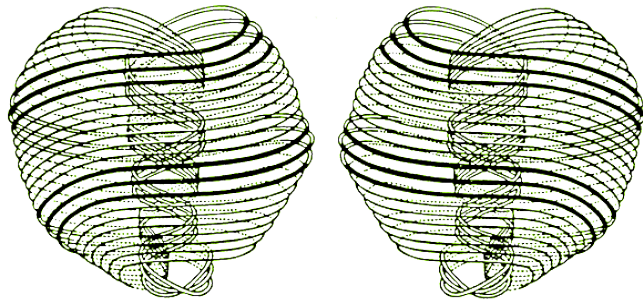
Positive and Negative chiral forms of UPA
